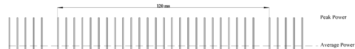
Figure 3. GSM Multiframe Showing Missing 26th Frame
